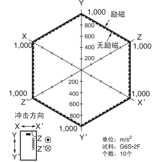
误动作冲击 G6S-2F(G)
